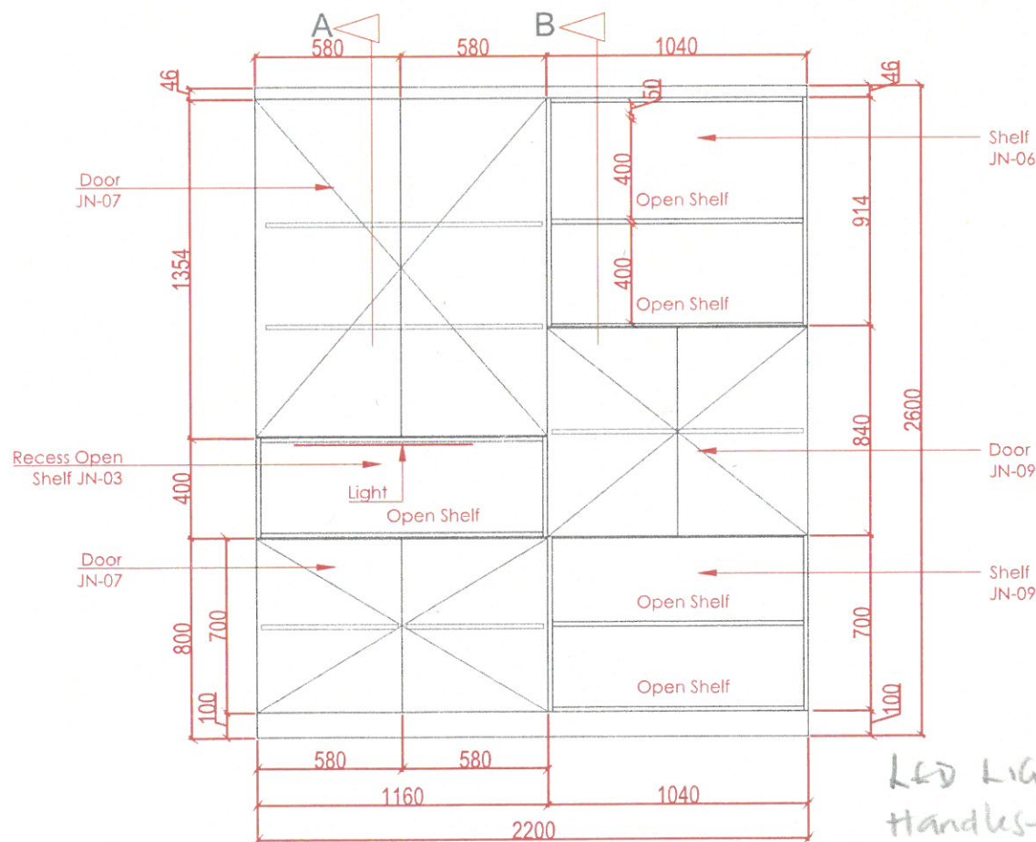
Elevation - Details
