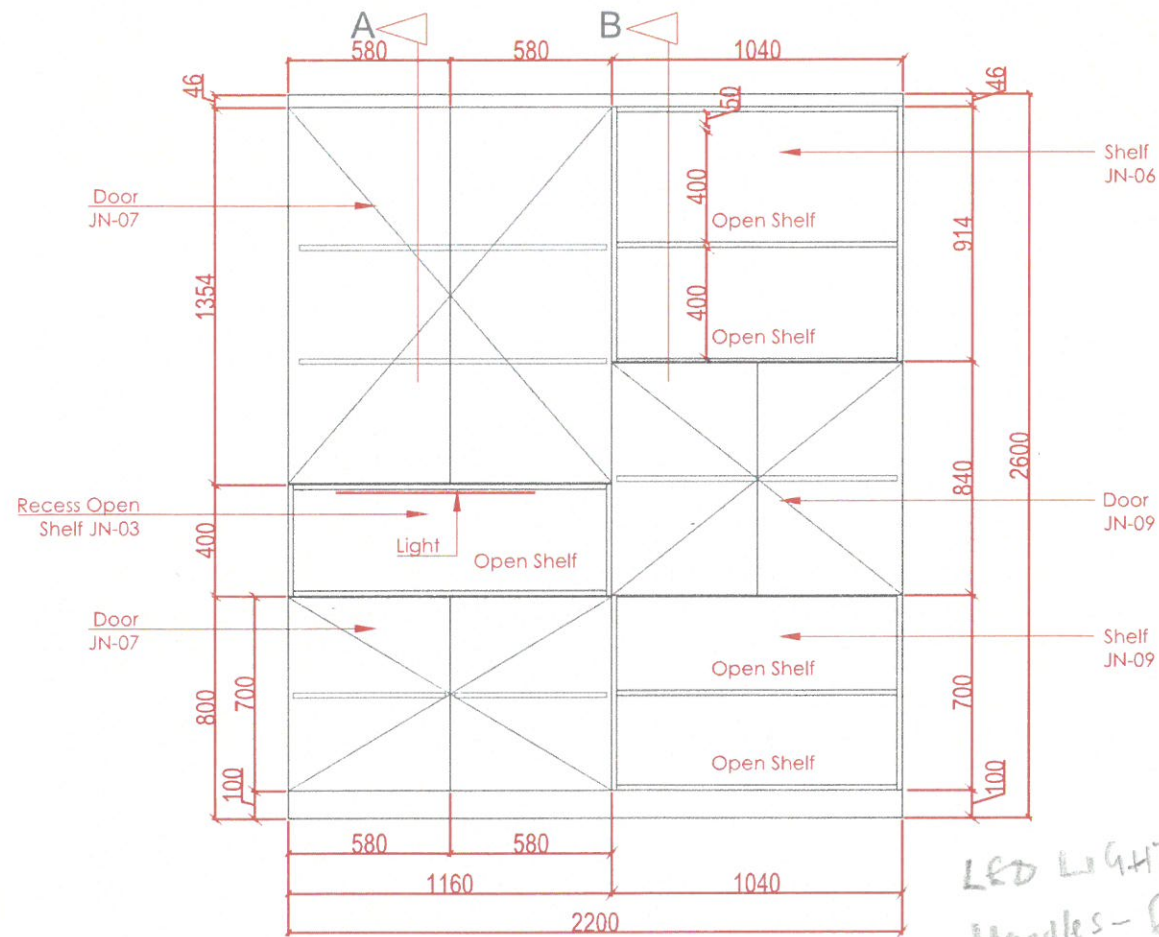
Elevation - Details
