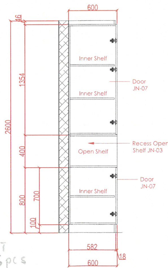
sectional details-A
