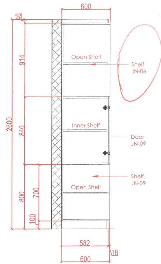
sectional details-B
