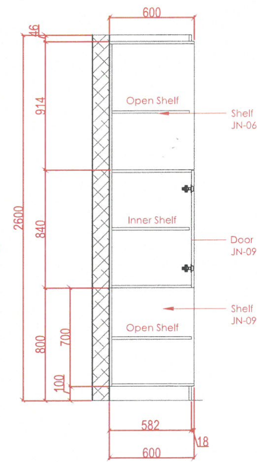
sectional details-B
