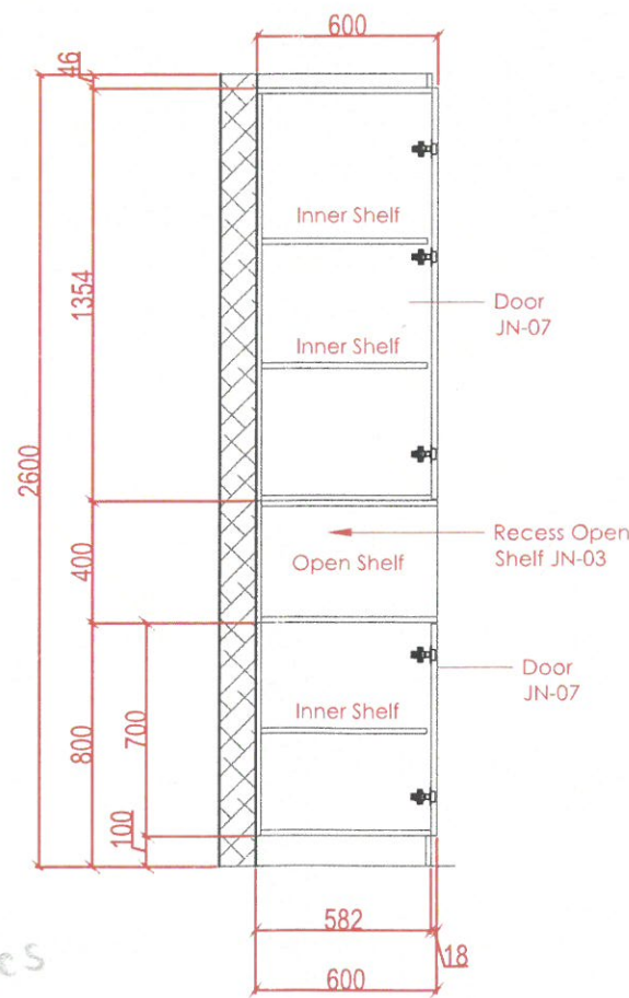
sectional details-A
